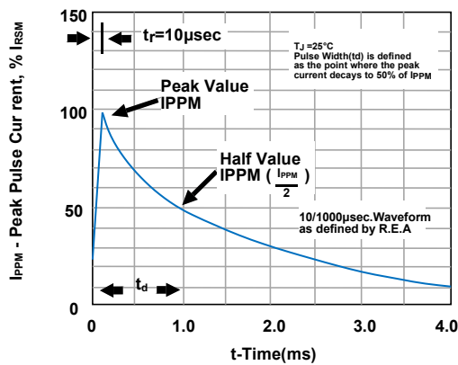
Figure 5 - Pulse Waveform
